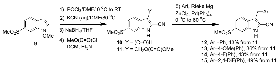
Scheme 3. Preparation of indoles 12–15 from indole methylcarbonate 11 .
